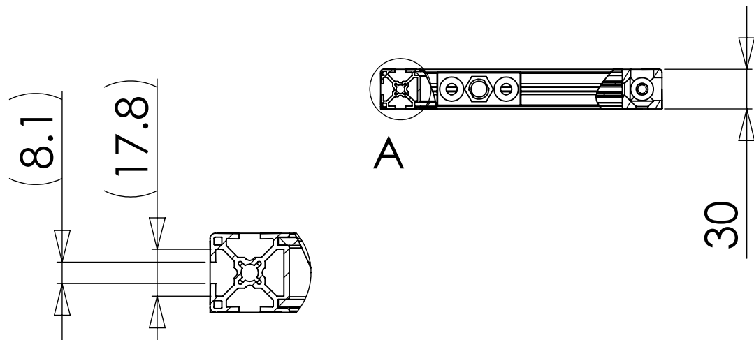
DETAIL A SCALE 1 : 2
